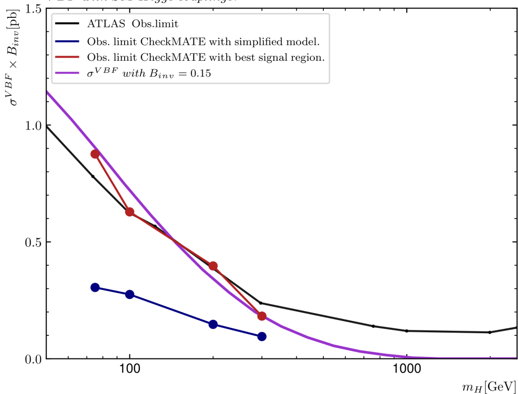
VBF with SM Higgs couplings.
